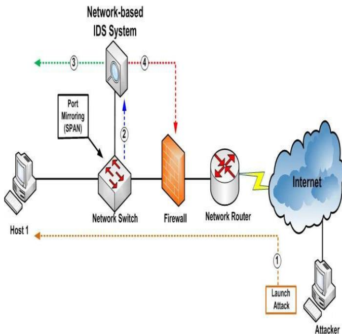
Figure 4: NIDS Architecture
