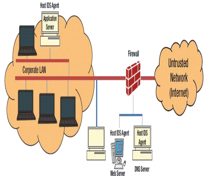
Figure 3: HIDS Architecture
