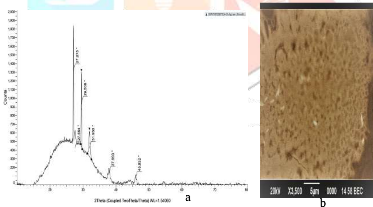
Figure 3: Mirabilis jalapa flower extract silver nanoparticles a) X-Ray Diffraction Ag (Coupled Two Theta/Theta); b) SEM micrograph of silver nanoparticles.
